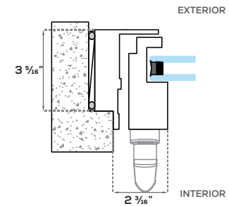
Hidden frame Horizontal Section
