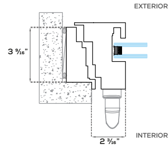
Hidden Frame Horizontal Section
