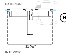
WIDE SASH + WIDE SASH
