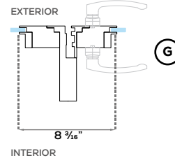
STANDARD SASH + STANDARD SASH
