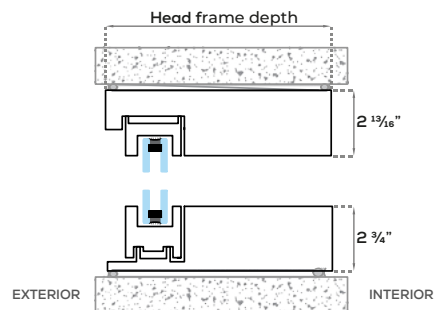
VERTICAL SECTION
