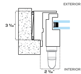
Hidden frame Horizontal Section
