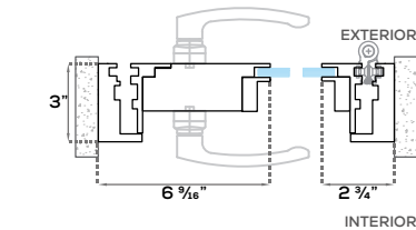
Option 1 Horizontal section
