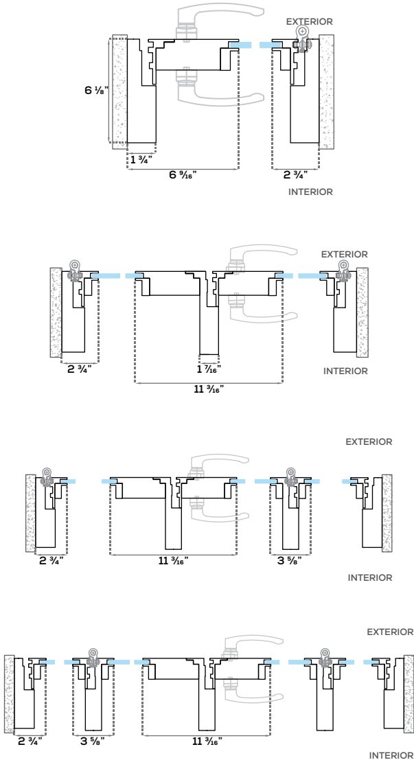
Option 2 Horizontal section
